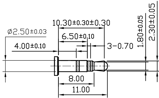
Ø2.5mm 3 POLE PLUG DETAIL DRAWING
