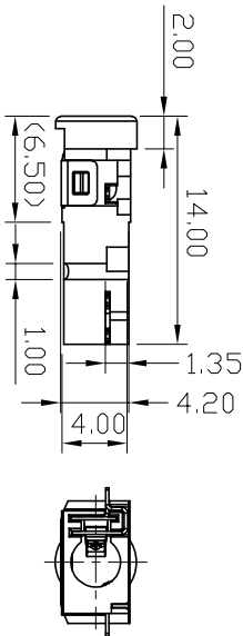
(ø3.50mm 4 POLE PLUG DETAIL DRAWING)
