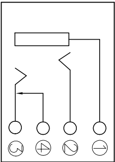
CIRCUIT
