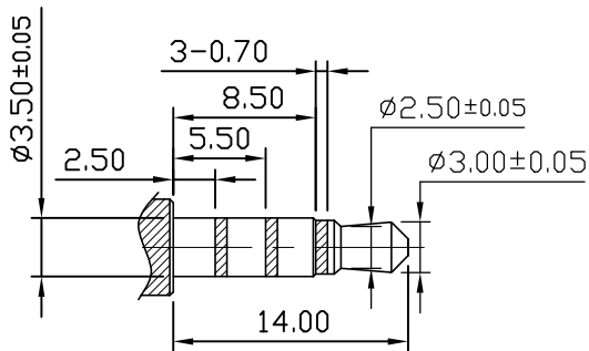
( \phi 3.50\text{mm} 4 POLE PLUG DETAIL DRAWING)
