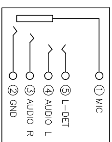
CIRCUIT
