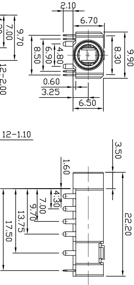
(ø4.40mm 5 POLE PLUG DETAIL DRAWING)
