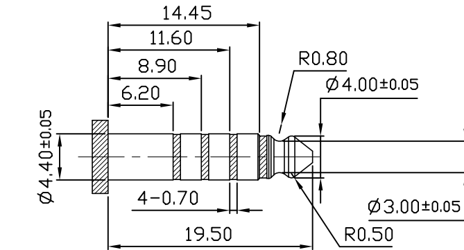
(Ø4.40mm 5 POLE PLUG DETAIL DRAWING)
