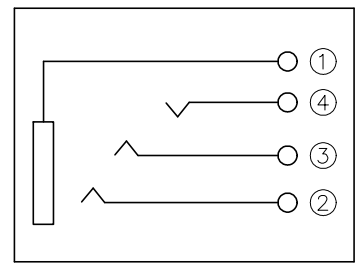
CIRCUIT
