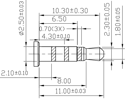
Ø2.50mm 4 POLE PLUG DETAIL DRAWING
