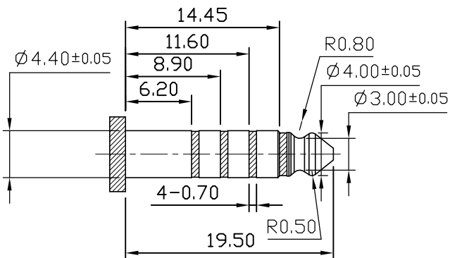
(Ø4.40mm 5 POLE PLUG DETAIL DRAWING)
