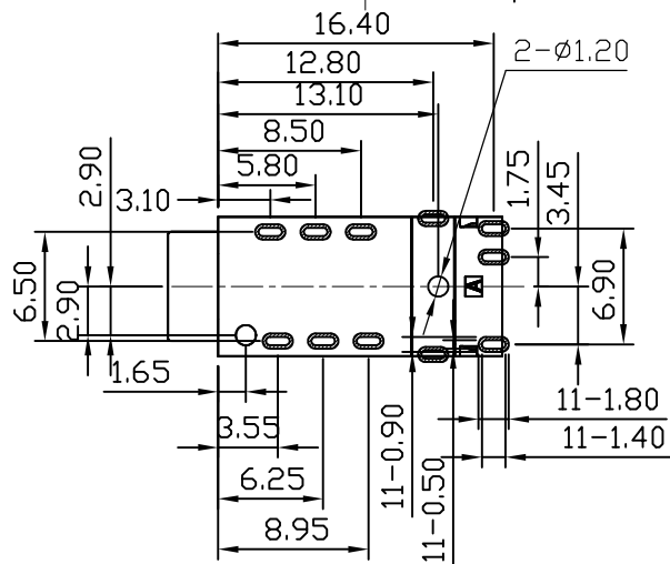
RECOMMENDED PCB LAYOUT TOP VIEW TOL:±0.05
