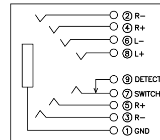
CIRCUIT
